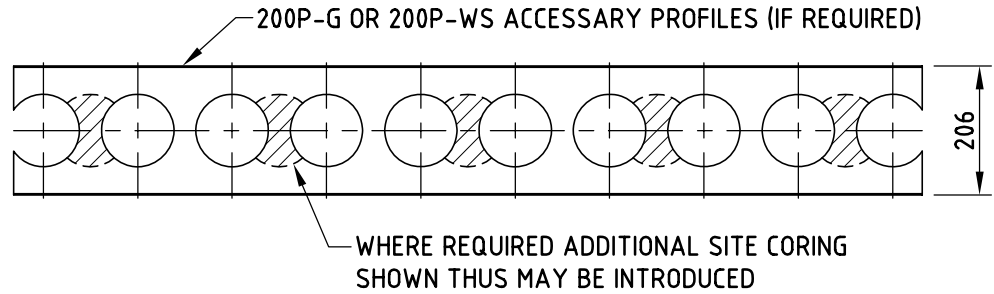
PLAN - WALL ASSEMBLY - WATERPROOF WALL RECOMMENDED FOR BUILDING BASEMENT/FACADE WALLS
